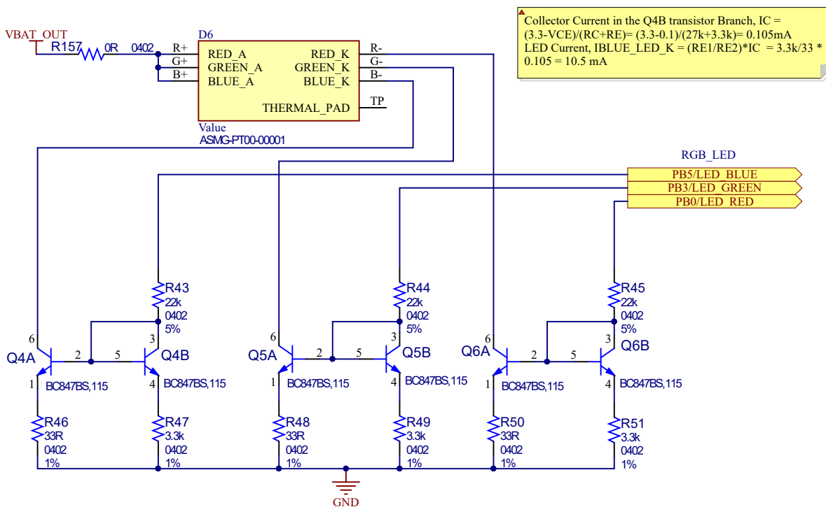
Figure 5-8. RGB LED
