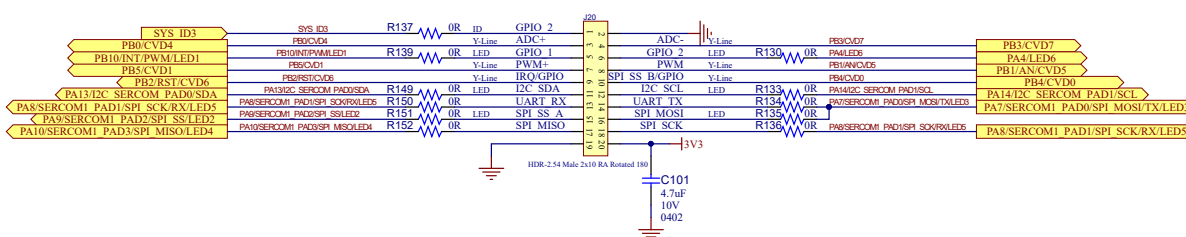
Figure 5-11. Xpro Header
