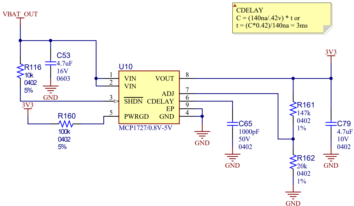
Figure 5-4. WBZ351PE Module 3.3V Regulator
