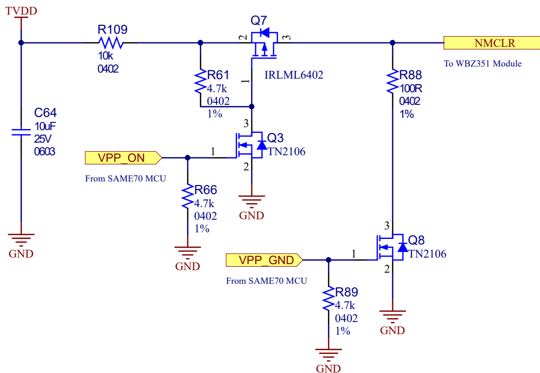
Figure 5-19. VDD Bleeder
