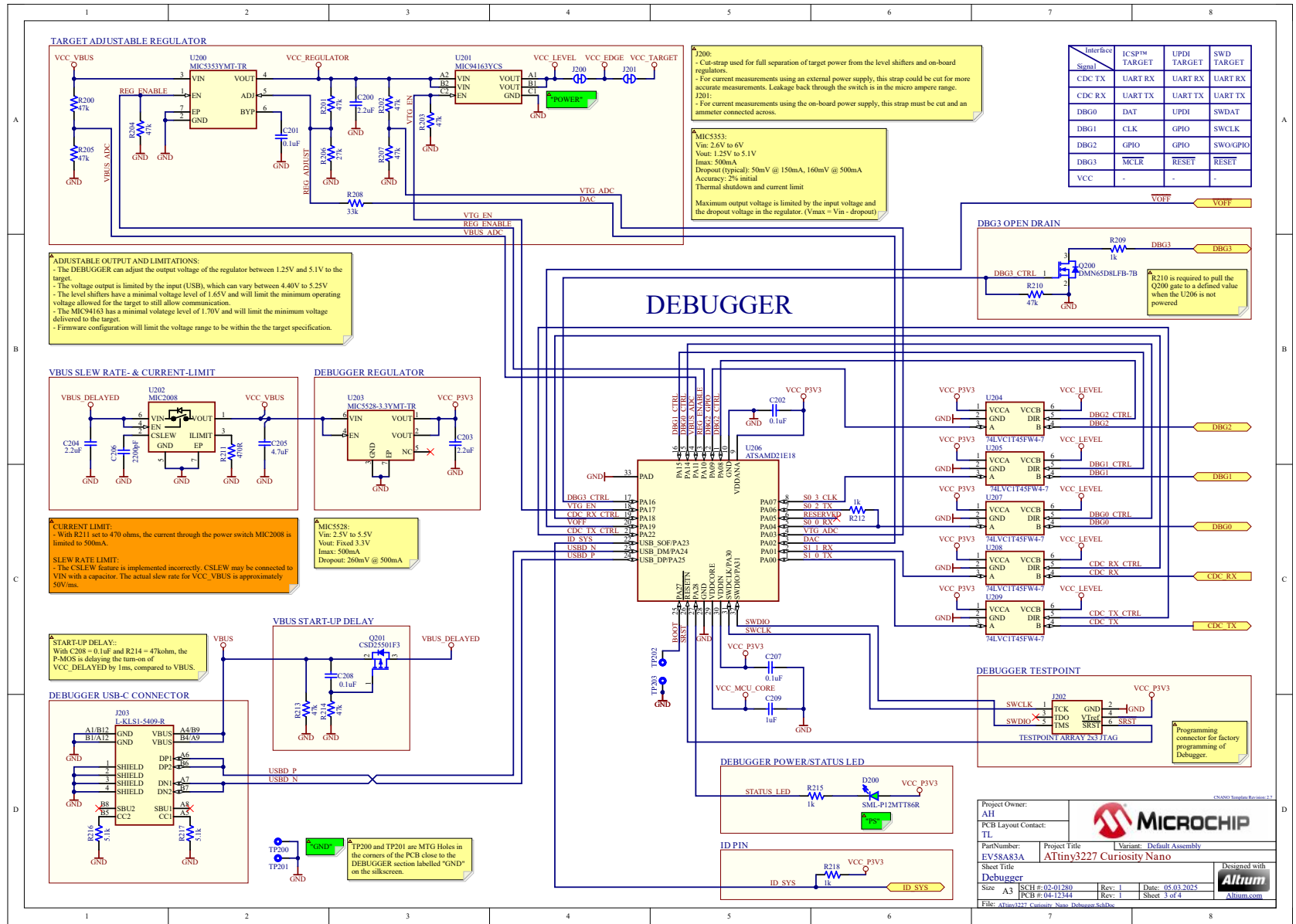
Figure 7-2. ATtiny3227 Curiosity Nano Debugger Schematic
