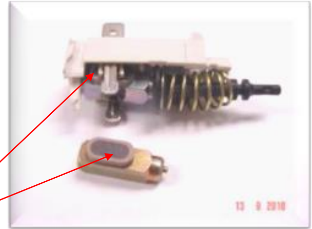
PTC wax motor
