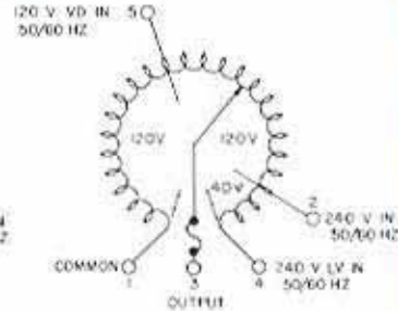
6020 Ganged Unit
