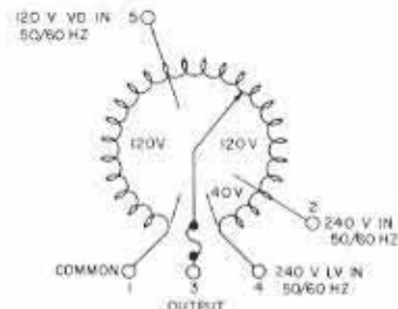
5021 Ganged Unit
