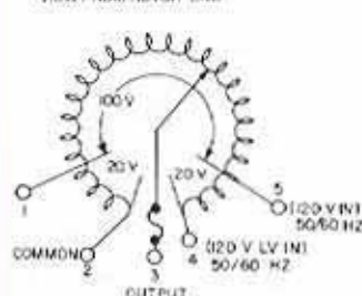
VIEW FROM ROTOR END
