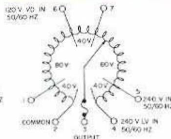
6020 Single Unit
