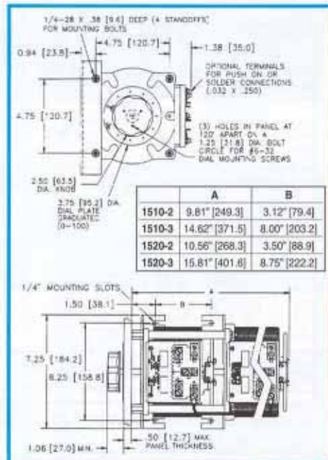
Manual Two- and Three-Ganged, Uncased
