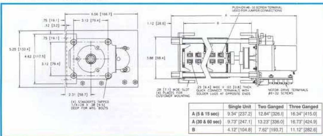
Motorized Single, Two and Three Ganged
