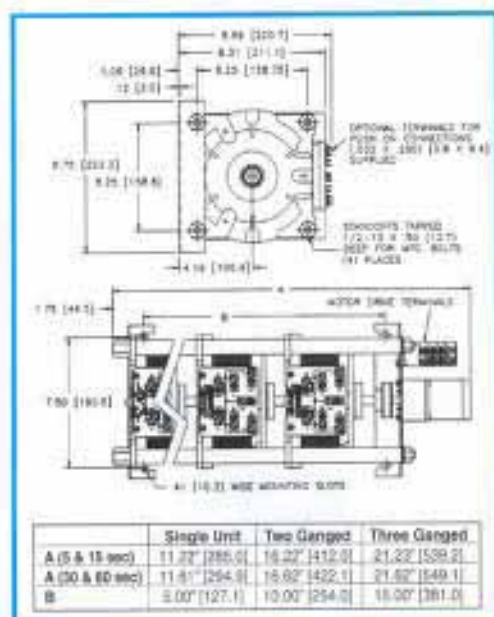
Motor-Driven Single, Two and Three-Ganged, Uncased
