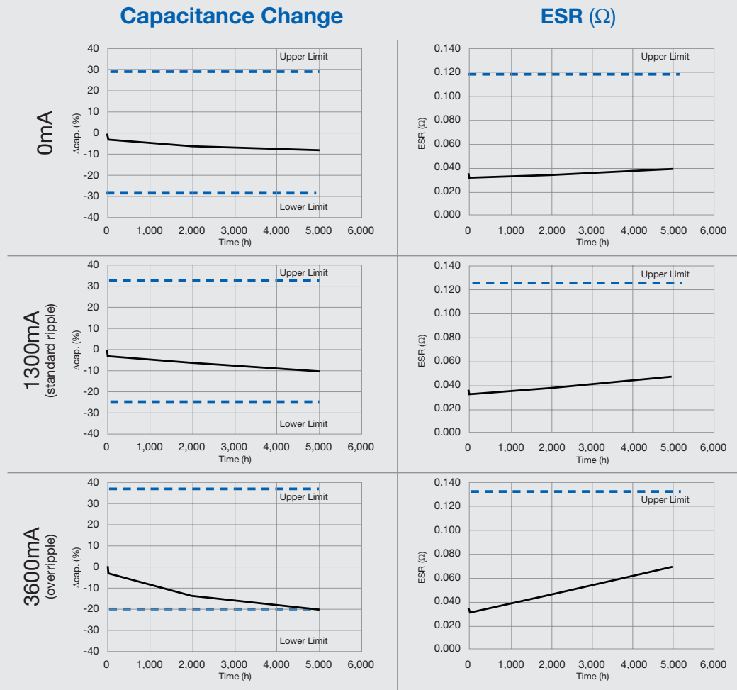
Figure 9 Hybrid capacitors exhibit high reliability when subjected to high ripple currents. In recent testing, the capacitors had the electrical characteristics at no load and rated ripple current (1300 mA) conditions. At three times the rated ripple current (3600 mA), the capacitor's electrical characteristics did change, but no shortage took place.
